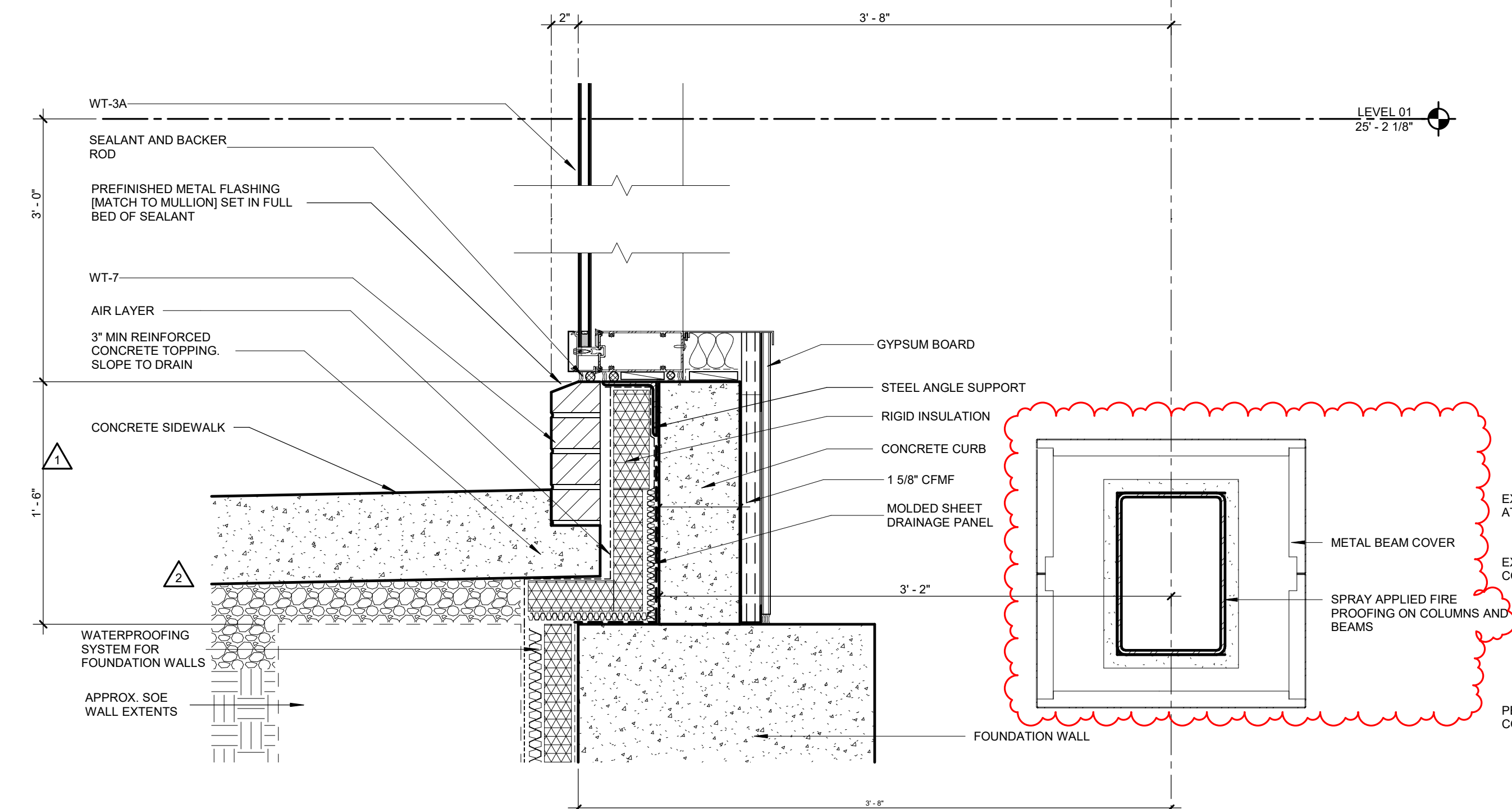
SECTION DETAIL - AT SE STAIR EAST CW TO SIDEWALK 05 1 1/2" = 1'-0"
