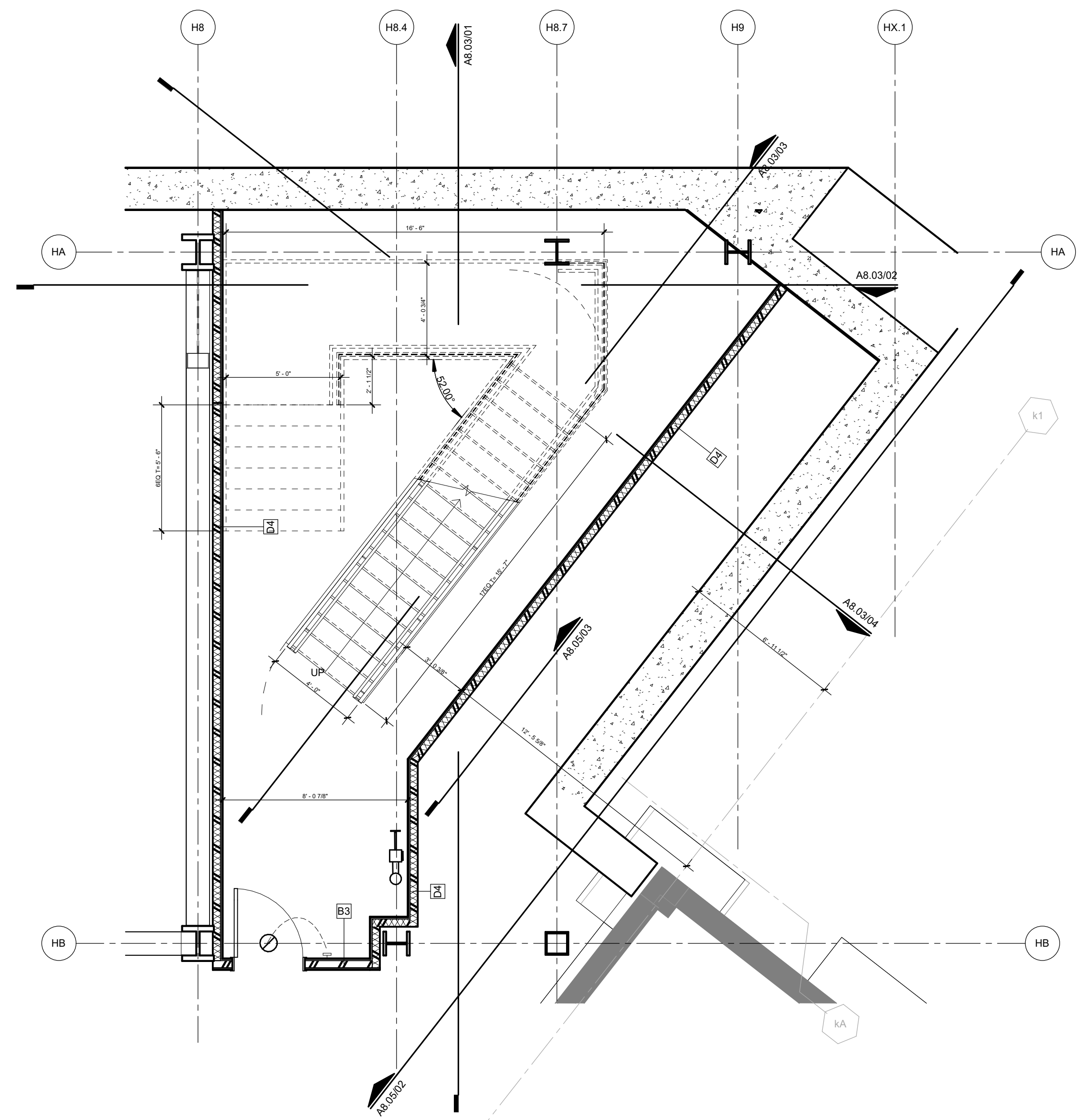
01 ENLARGED PLAN - LEVEL BASEMENT 1/4" = 1'-0"
