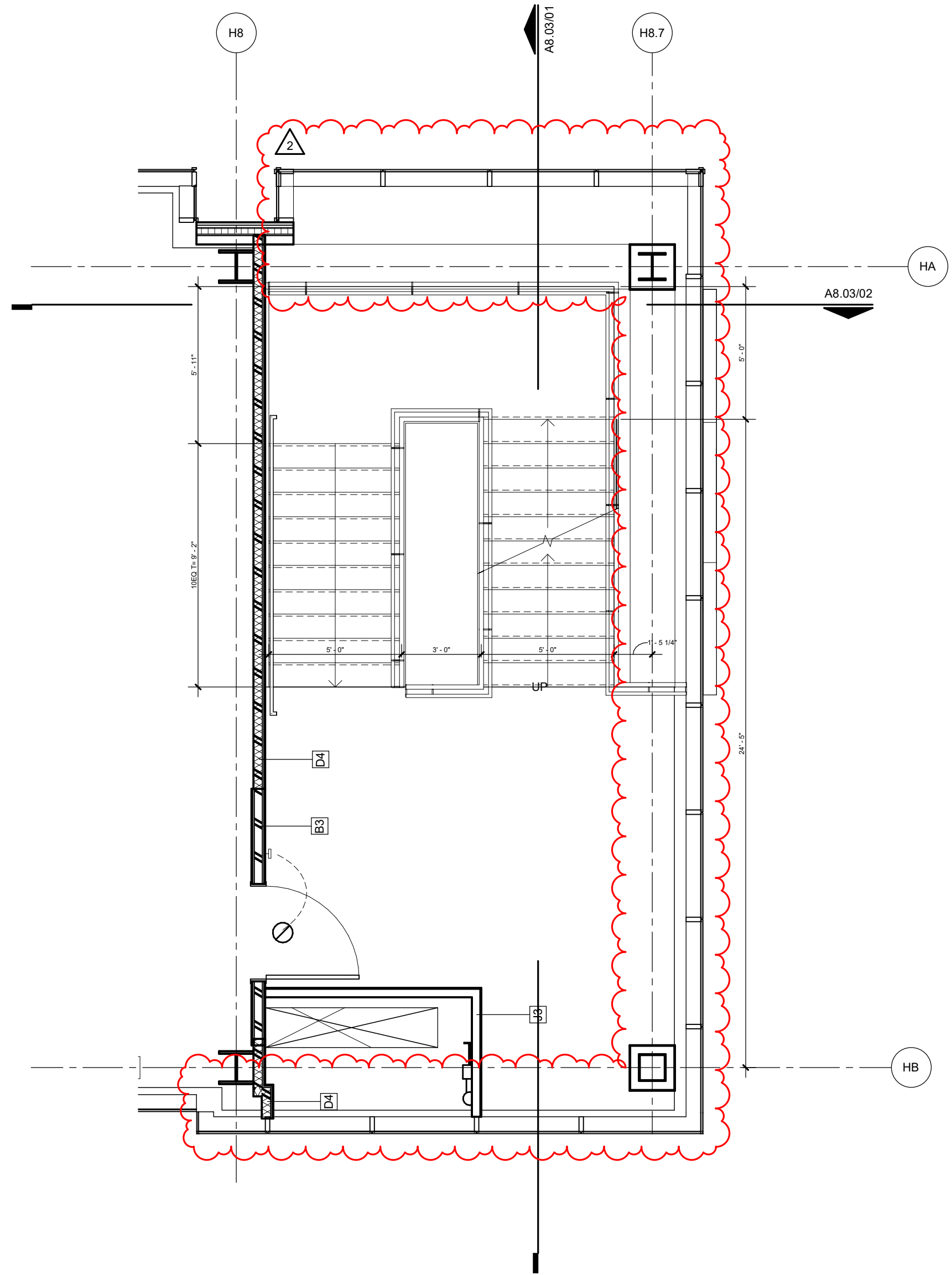
06 ENLARGED PLAN - ST02 - LEVEL 10 1/4" = 1'-0"
