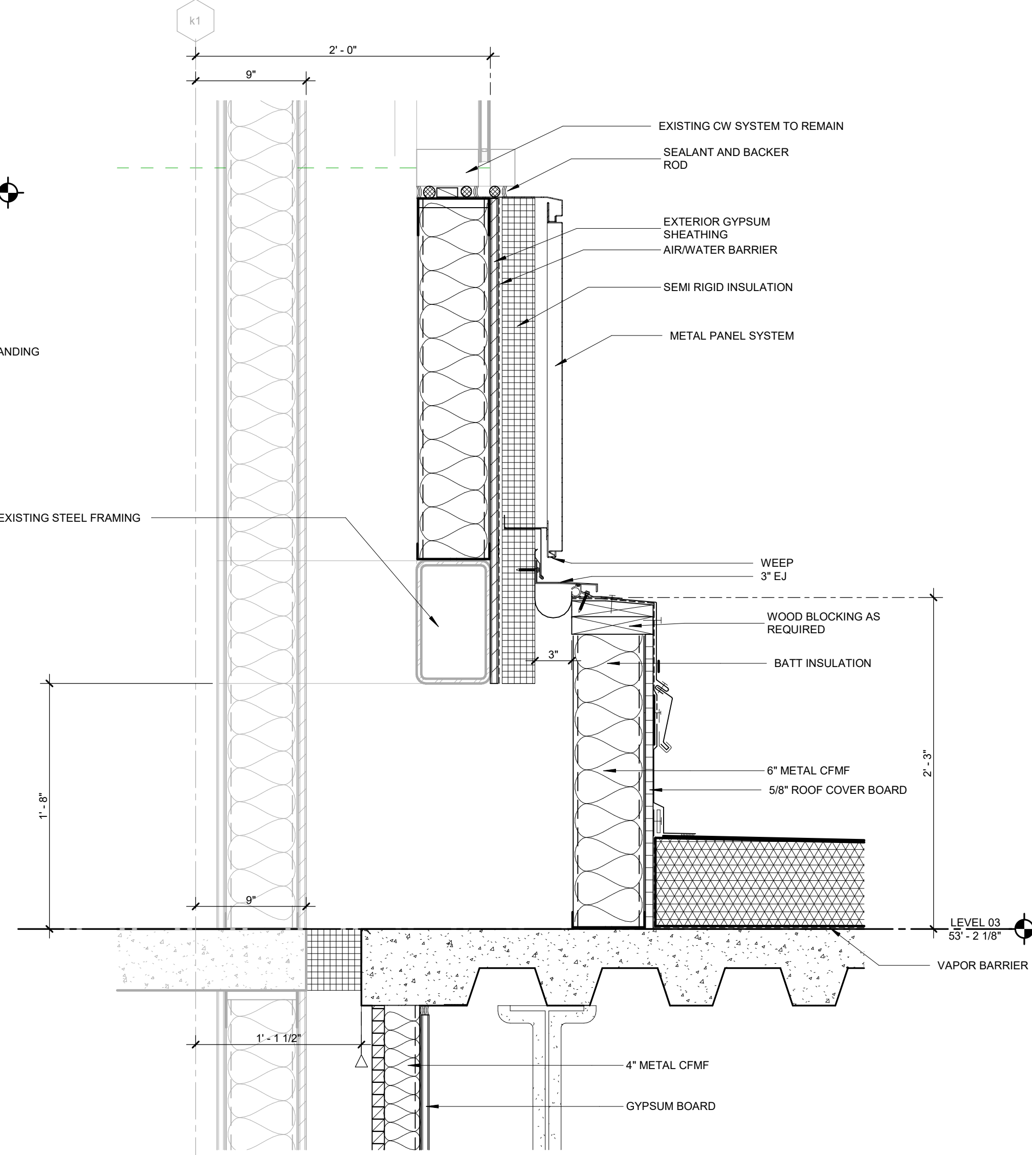
SECTION DTL - LVL 03 ROOF TRANSITION TO KEELMEN TOWER 03 1 1/2" = 1'-0"
