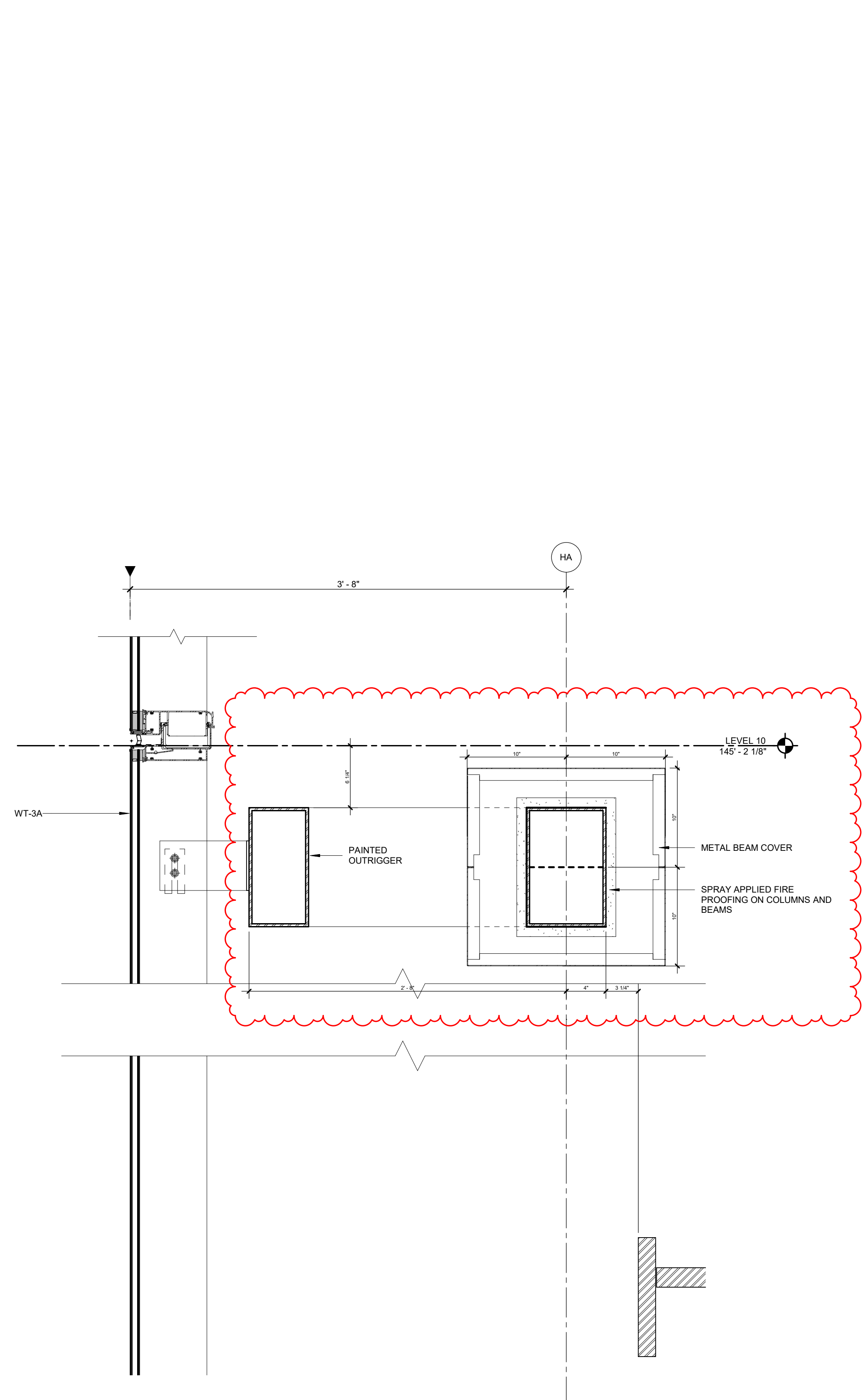
01 SECTION DTL - SE STAIR TOWER EAST CW TO STAIR INTERMEDIATE LANDING, TYP 1 1/2" = 1'-0"
