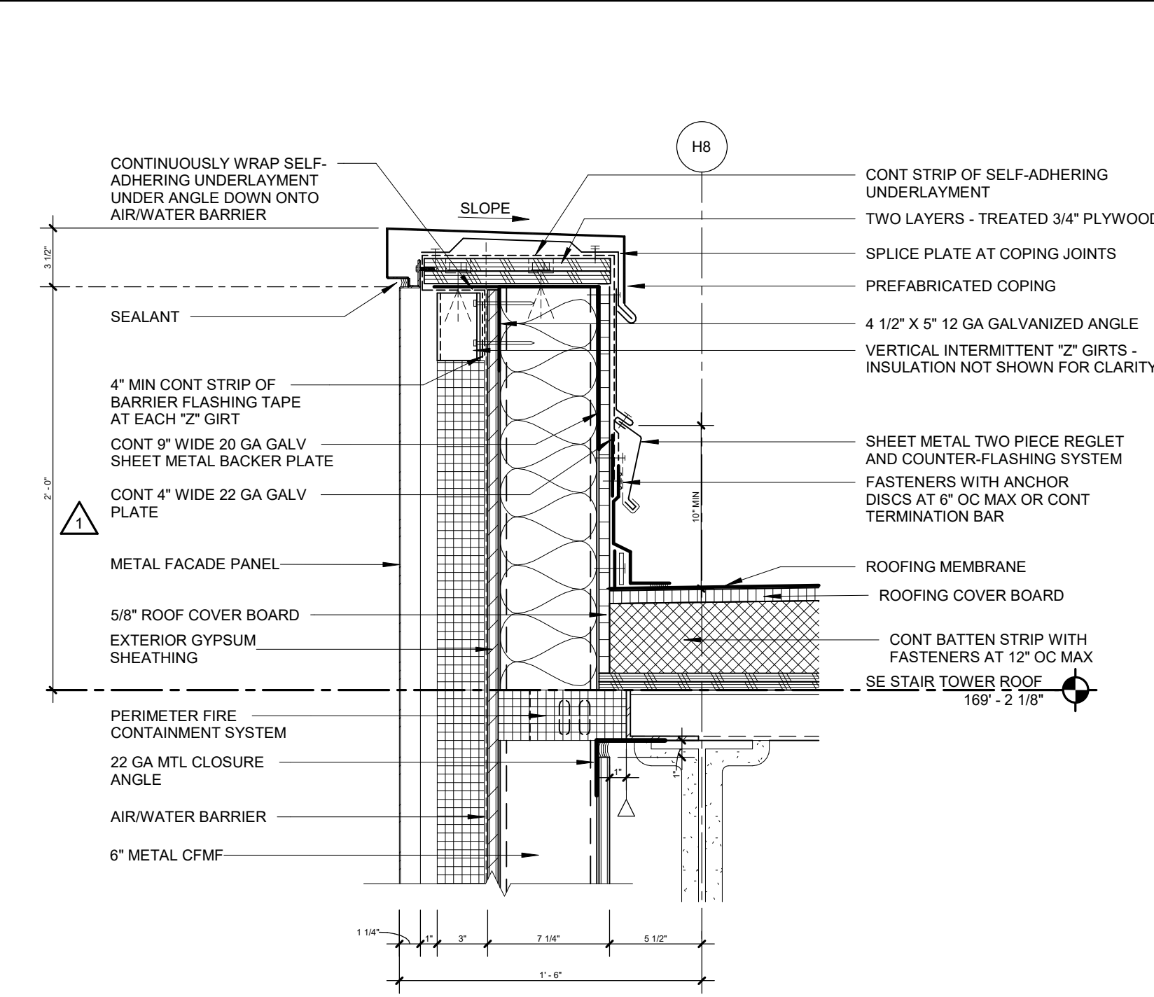
05 SECTION DTL - SE STAIR TOWER EAST NORTH METAL PANEL WALL PARAPET 1 1/2" = 1'-0"
