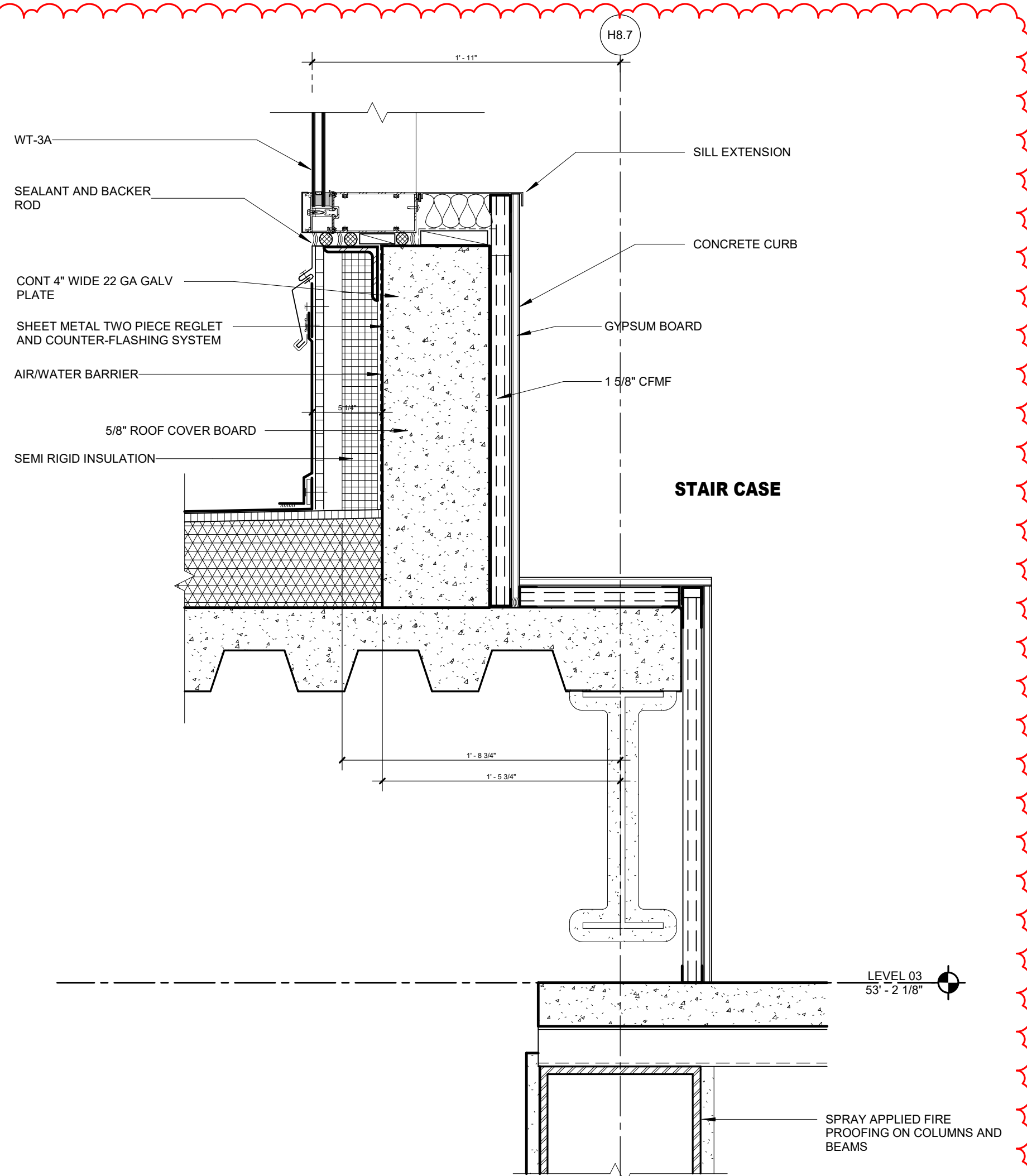
06 SECTION DTL - SE STAIR TOWER SOUTH CW TO BRIDGE ROOF 1 1/2" = 1'-0"
