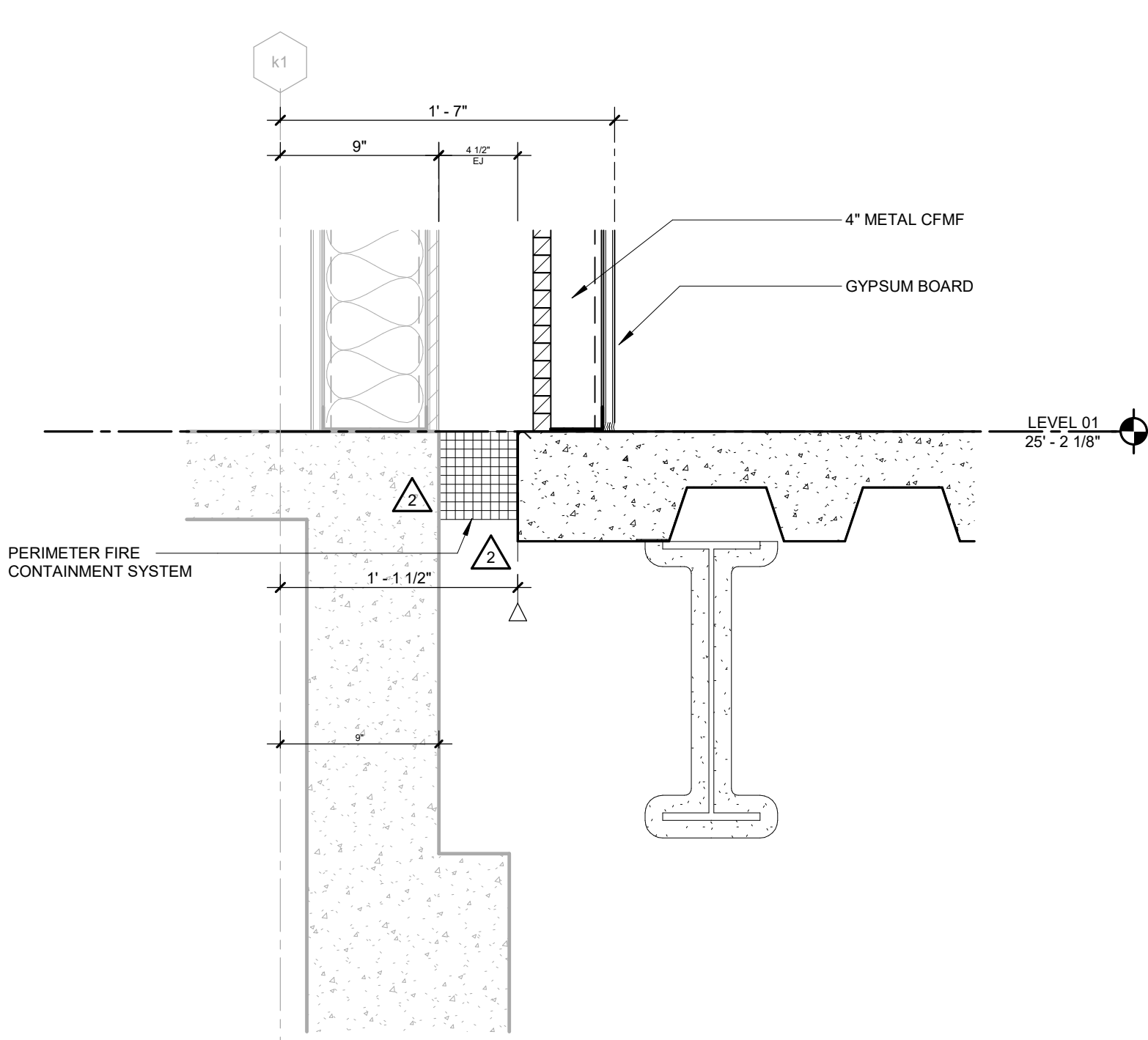
SECTION DTL - AT LEVEL 01 SOUTH SLAB EDGE TRANSITION TO KEELMEN 01 1 1/2" = 1'-0"
