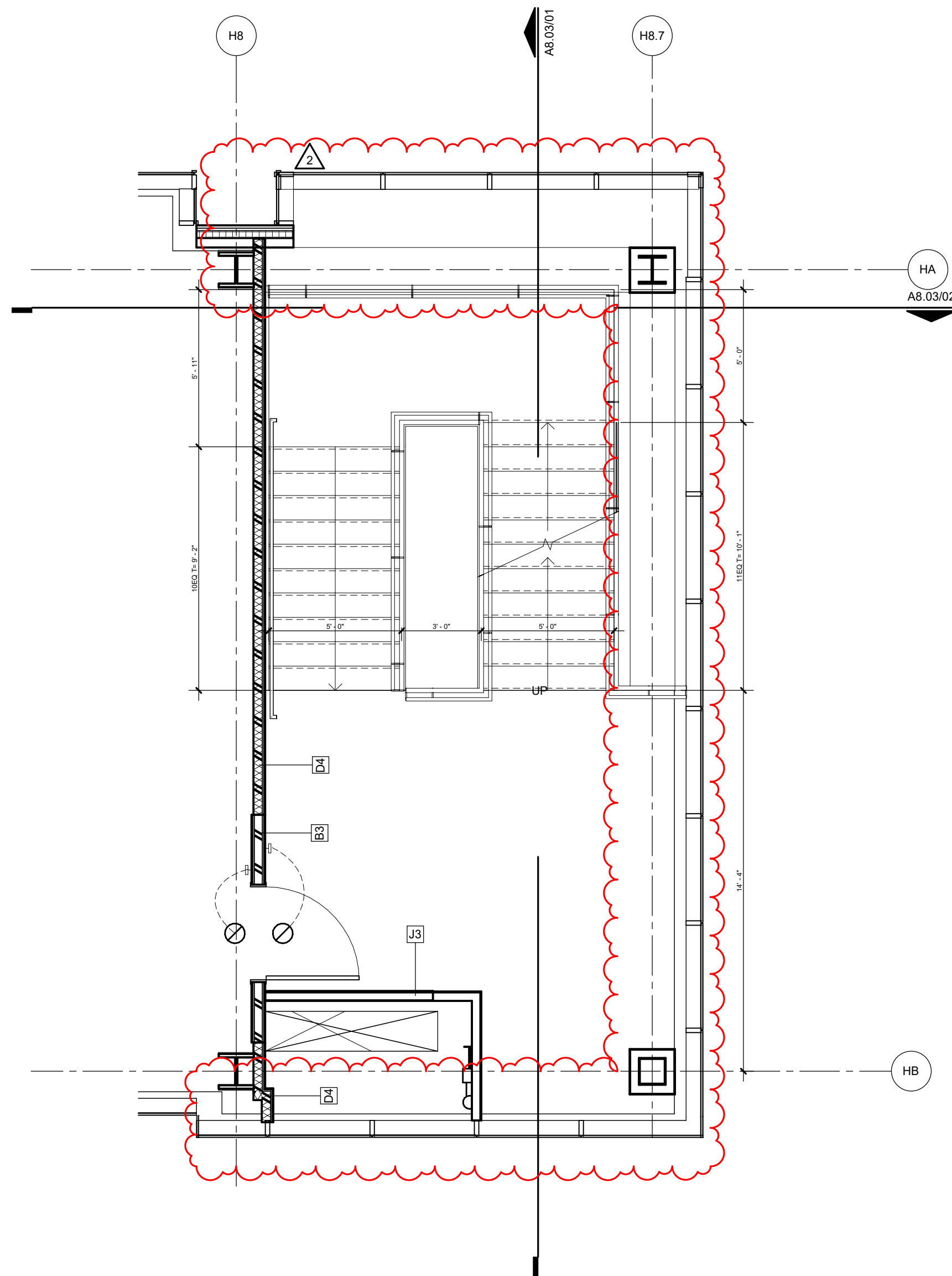
05 ENLARGED PLAN - ST02 - TYPICAL LEVEL 04-09 1/4" = 1'-0"
