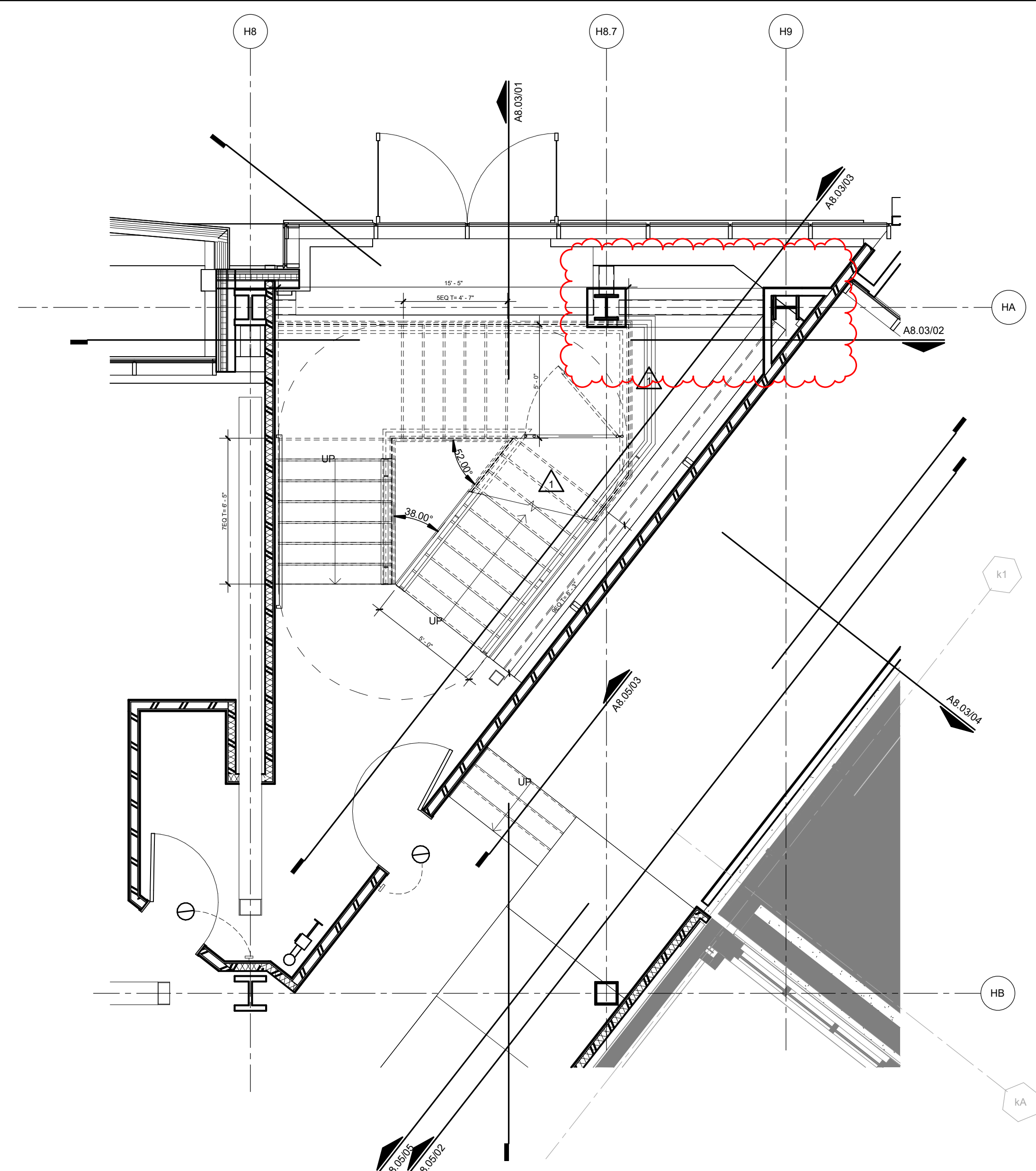
02 ENLARGED PLAN - ST02 - LEVEL 01 1/4" = 1'-0"
