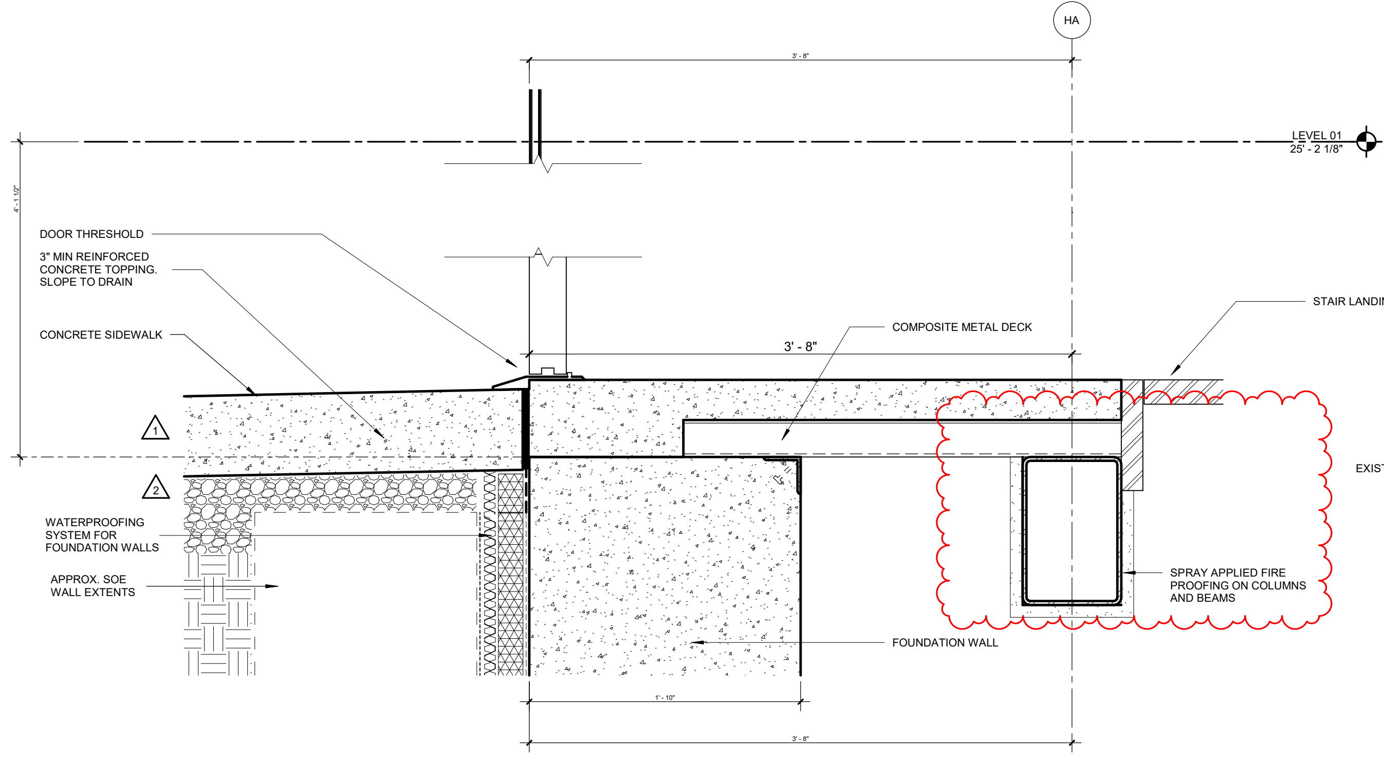
SECTION DTL - SE STAIR TOWER STAIR LANDING TO SIDEWALK 06 1 1/2" = 1'-0"
