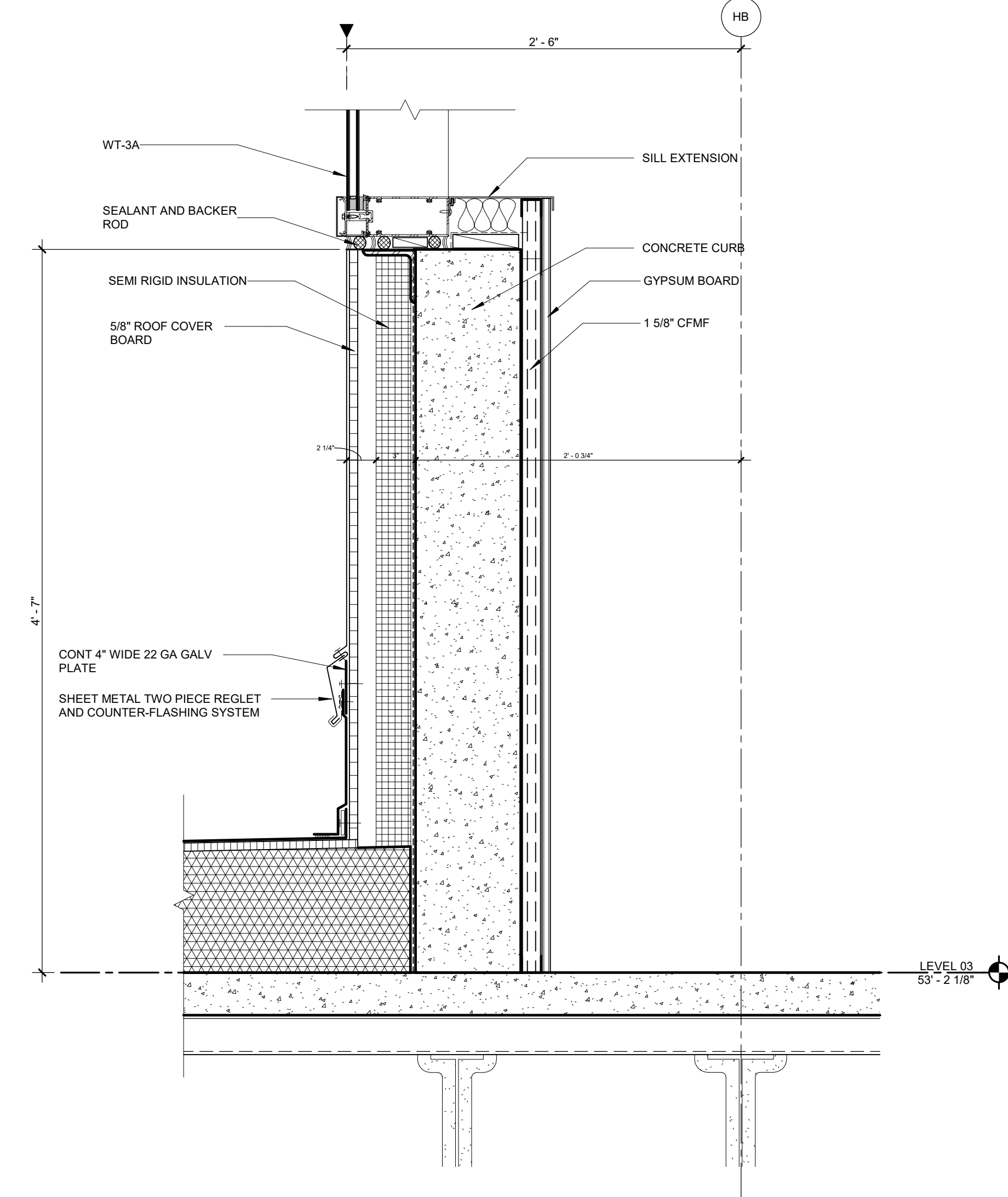
03 SECTION DTL - SE STAIR TOWER WEST CW TO ROOF 1 1/2" = 1'-0"
