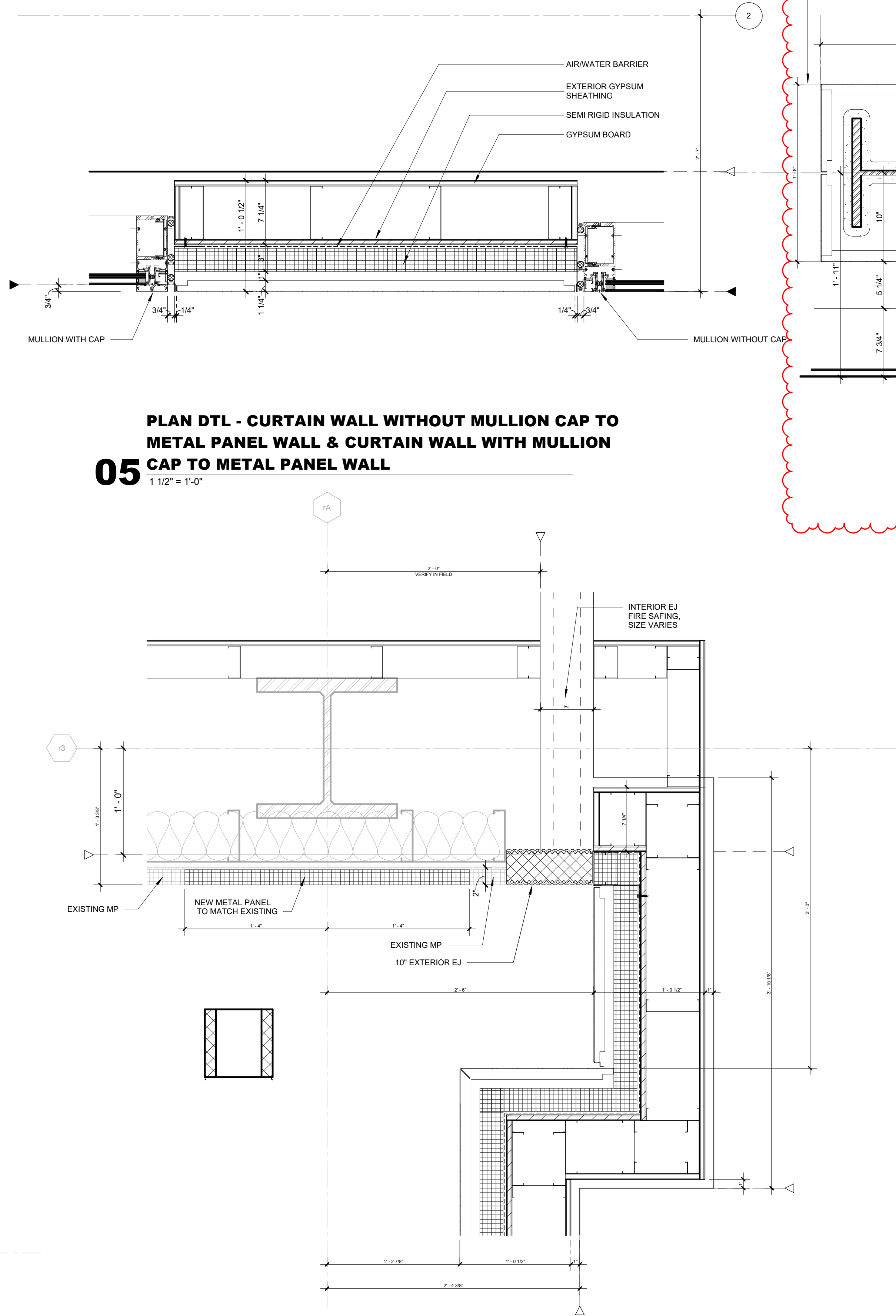
04 PLAN DETAIL - AT EXPANSION JOINT OF WEST TOWER A MEETS ROBERTS 1 1/2" = 1'-0"
