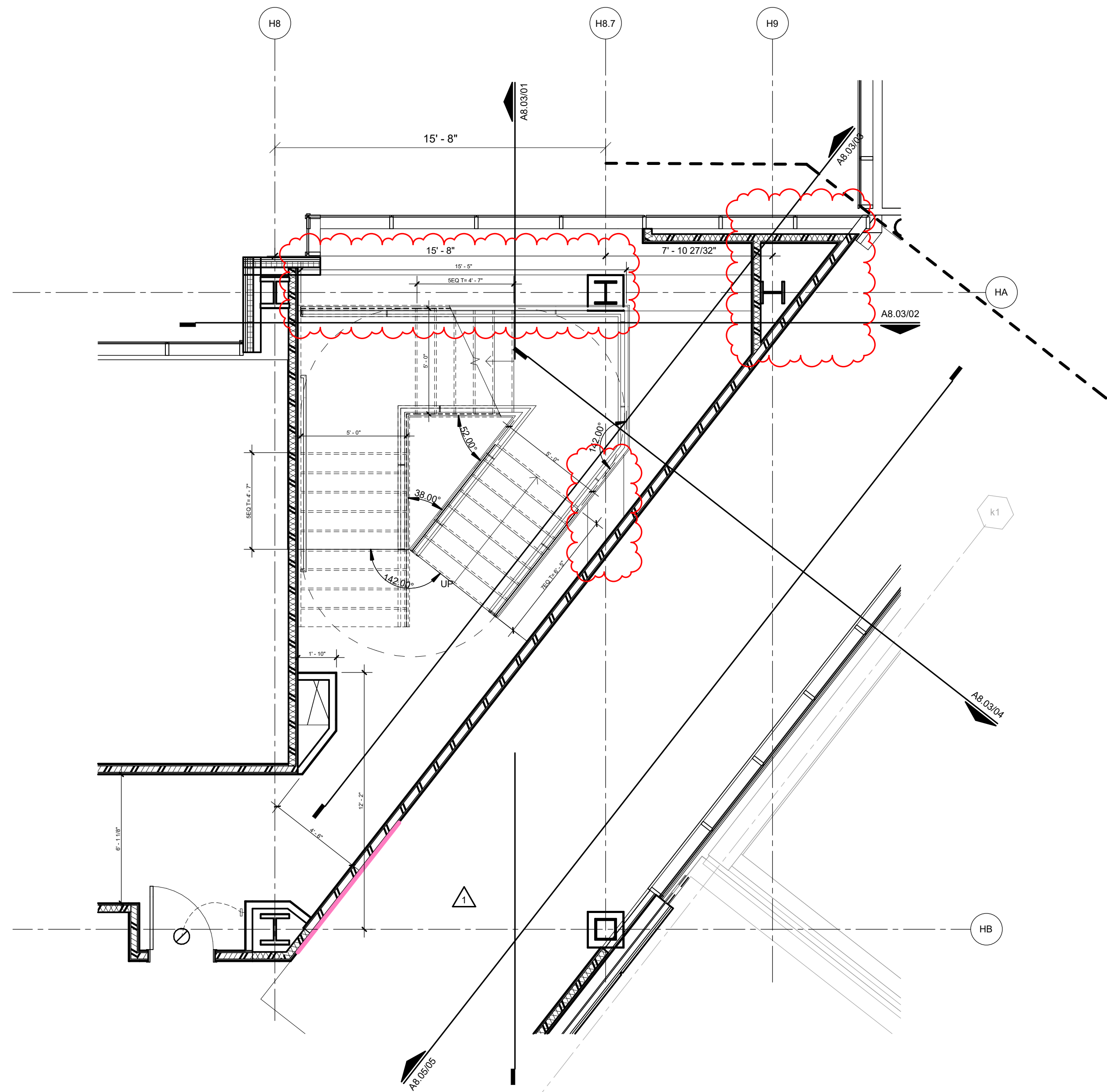
04 ENLARGED PLAN - ST02 - LEVEL 03 1/4" = 1'-0"
