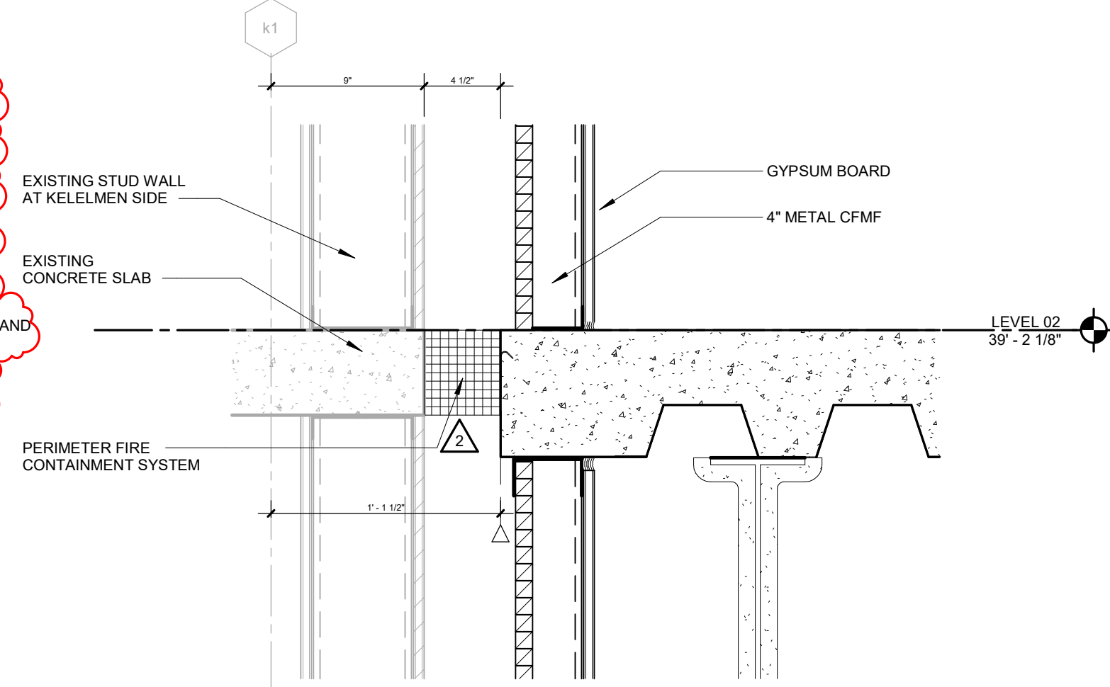
SECTION DETAIL - AT LEVEL 02 SOUTH SLAB EDGE TRANSITION TO KEELMEN 02 1 1/2" = 1'-0"
