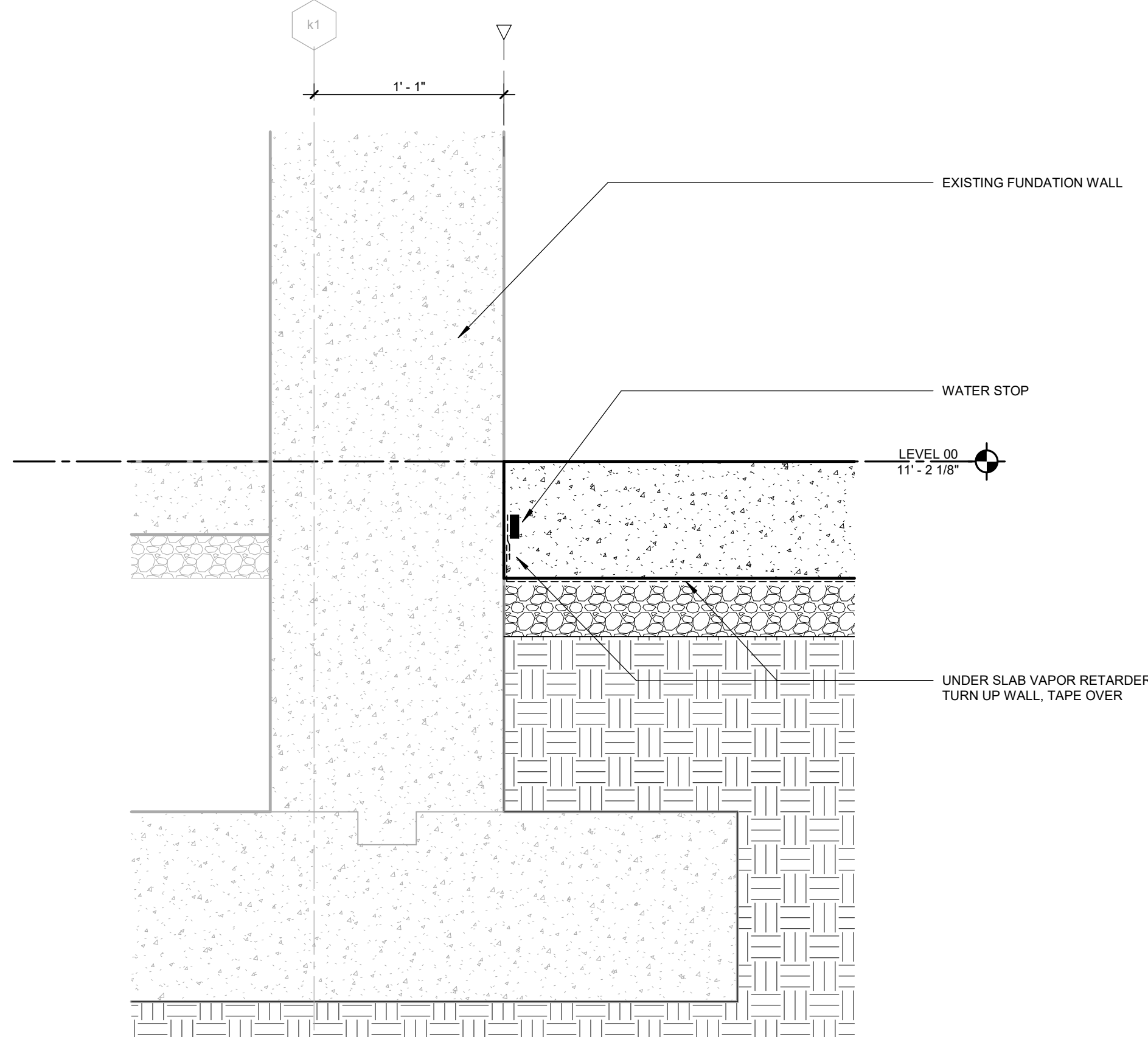
SECTION DETAIL - AT TOWER A TO ROBERTS AT LEVEL 00 CONDITION 01 04 1 1/2" = 1'-0"
