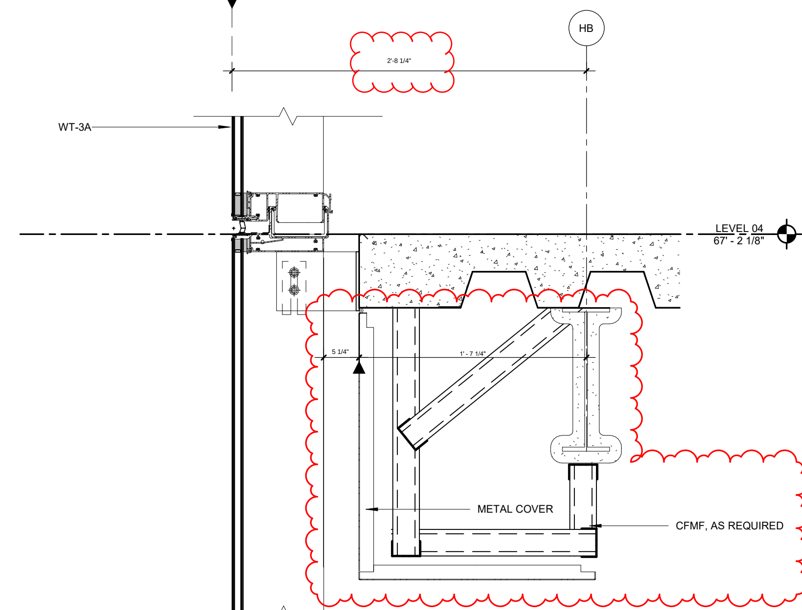
05 SECTION DTL - SE STAIR TOWER EAST NORTH METAL PANEL WALL PARAPET 1 1/2" = 1'-0"
