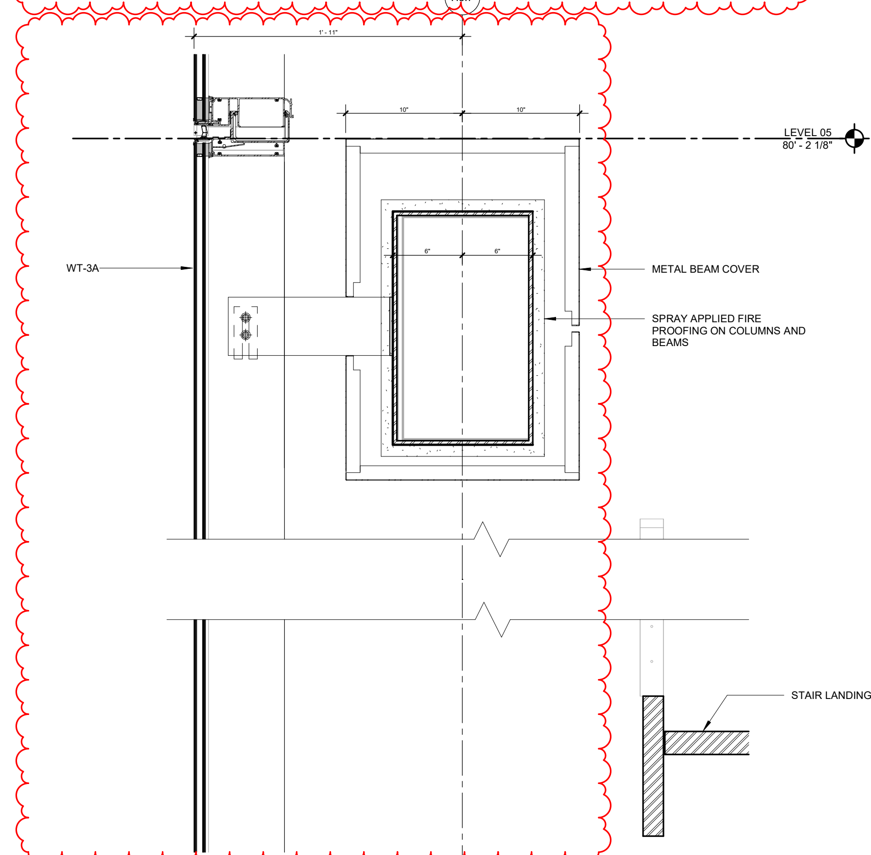
07 SECTION DTL - SE STAIR TOWER SOUTH CW TO STAIR INTERMEDIATE LANDING 1 1/2" = 1'-0"
