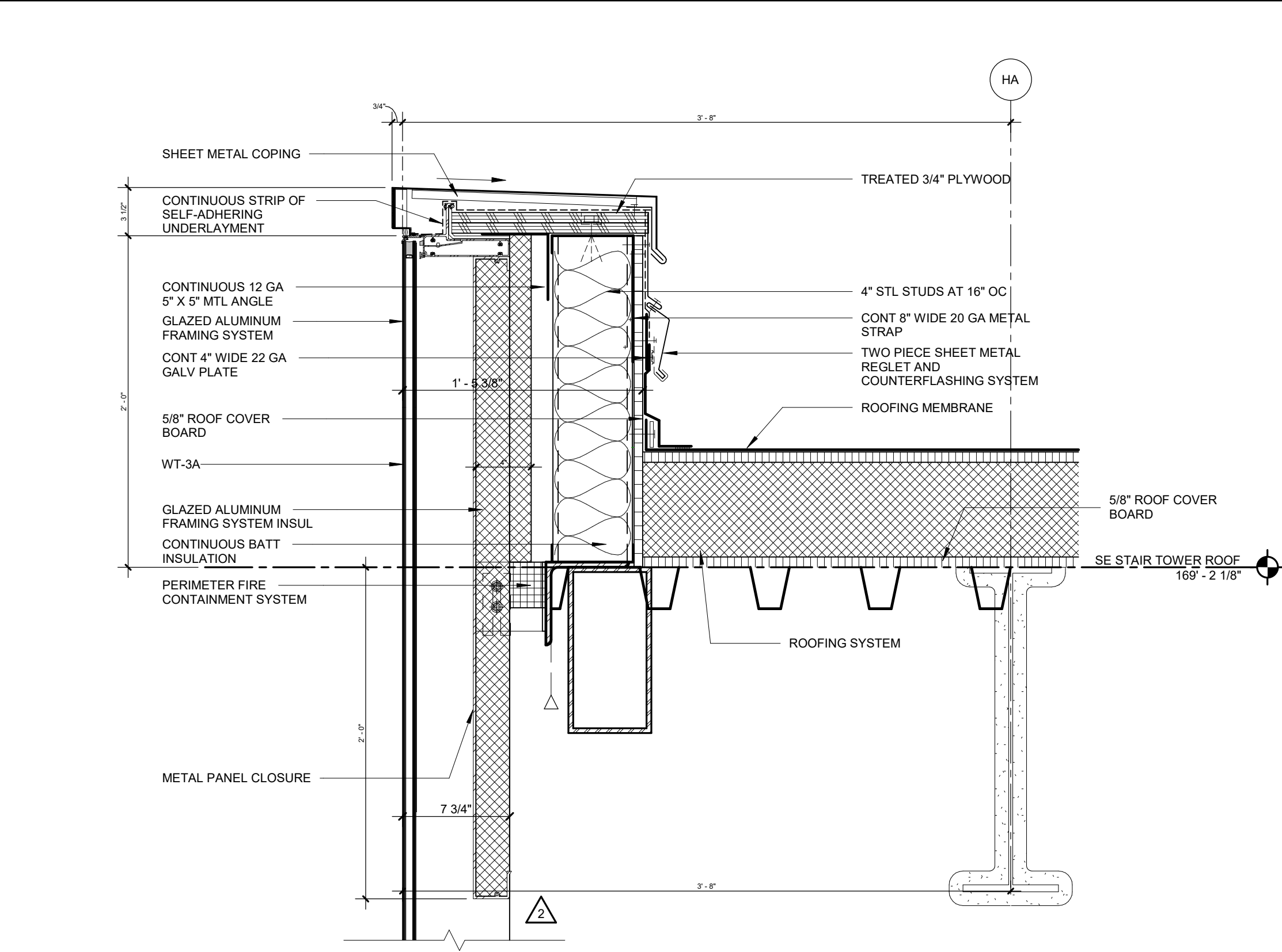
02 SECTION DTL - SE STAIR TOWER EAST CW PARAPHET 1 1/2" = 1'-0"
