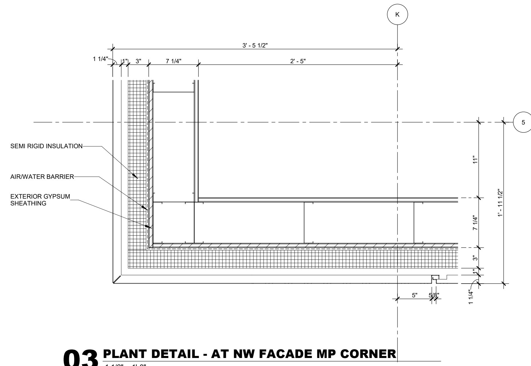
03 PLANT DETAIL - AT NW FACADE MP CORNER 1 1/2" = 1'-0"
