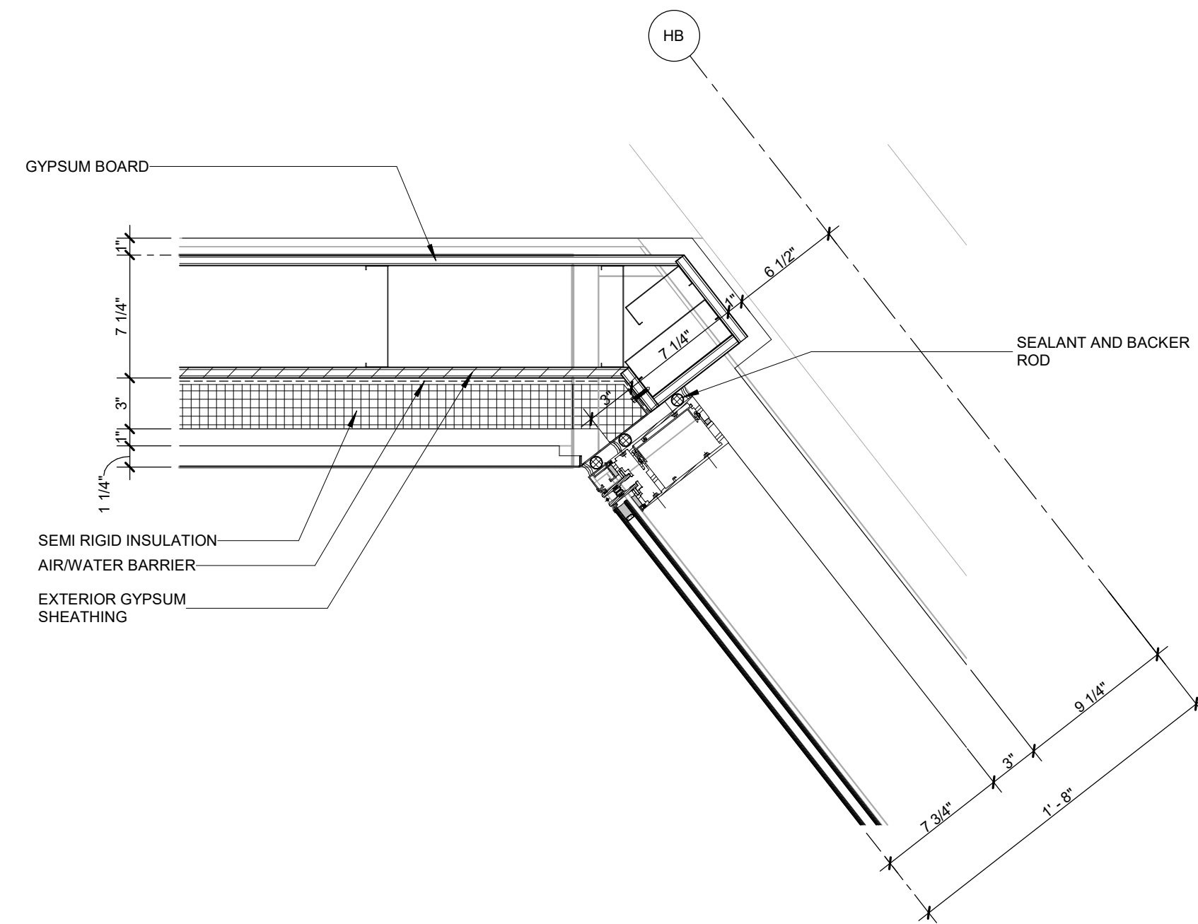
01 PLAN DTL - SE STAIR TOWER CURTAIN WALL TO SOUTH FACADE METAL PANEL WALL 1 1/2" = 1'-0"
