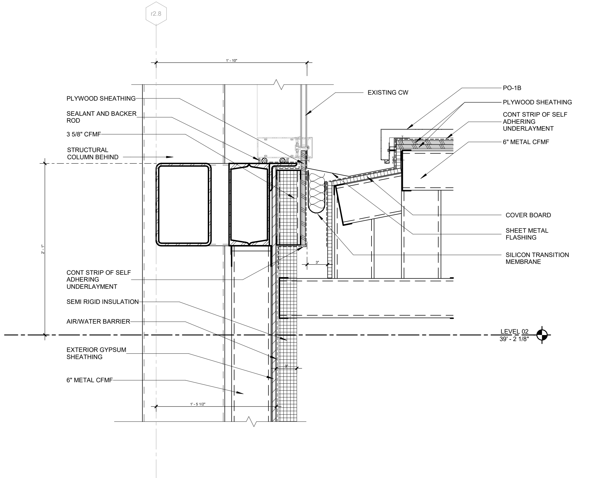
SECTION DETAIL - AT ROBERTS EXISTING CURTAIN WALL TO CONFERENCE CENTER FRAME ABOVE ENTRANCE 08 1 1/2" = 1'-0"
