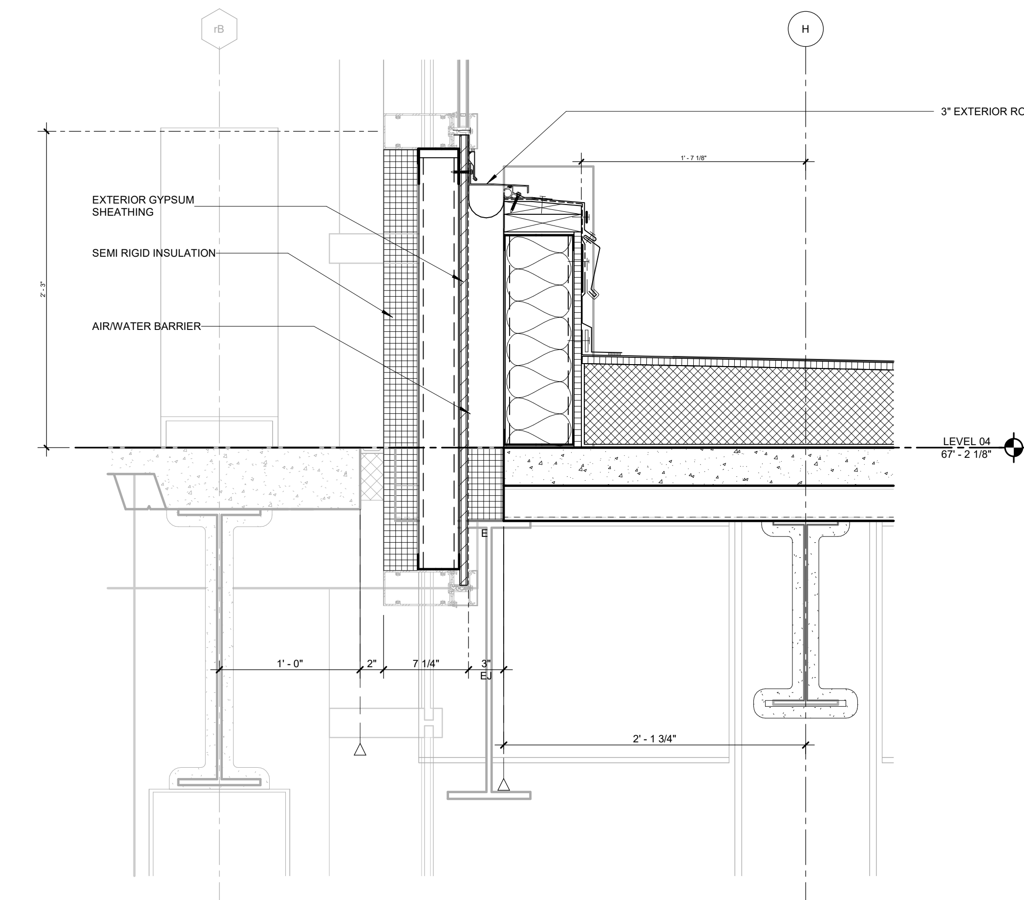
SECTION DETAIL - AT LEVEL 04 ROOF TO ROBERTS EXPANSION JOINT 07 1 1/2" = 1'-0"
